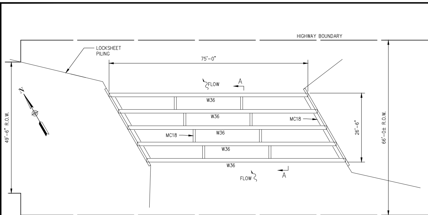
FRAMING PLAN NOT TO SCALE
