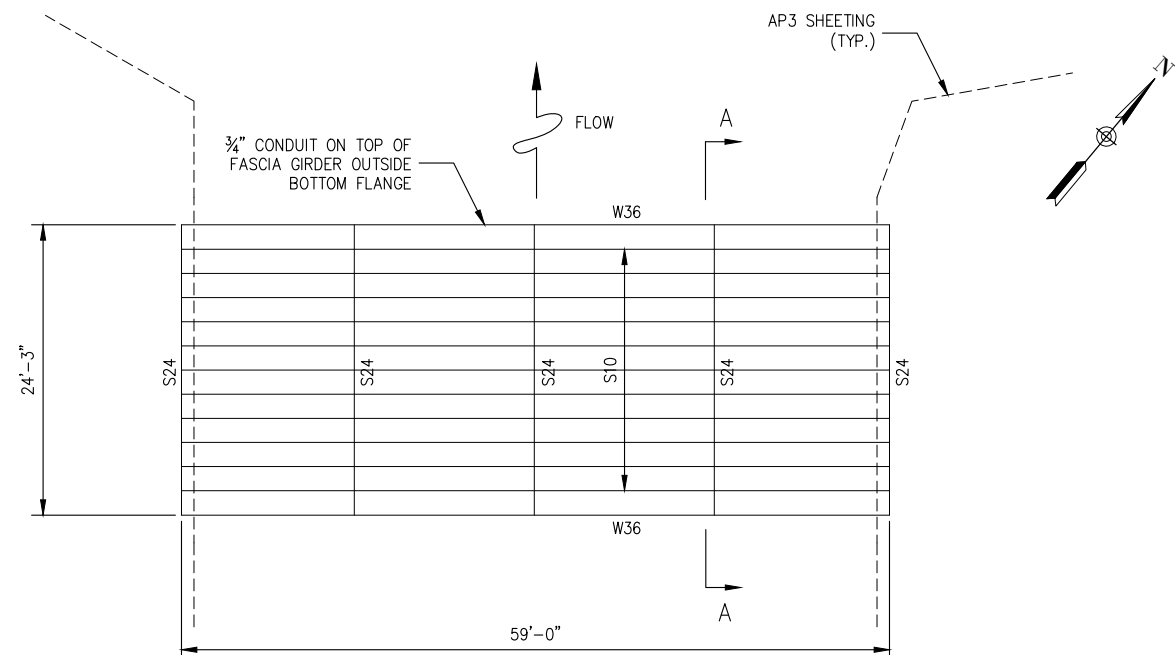
FRAMING PLAN NOT TO SCALE
