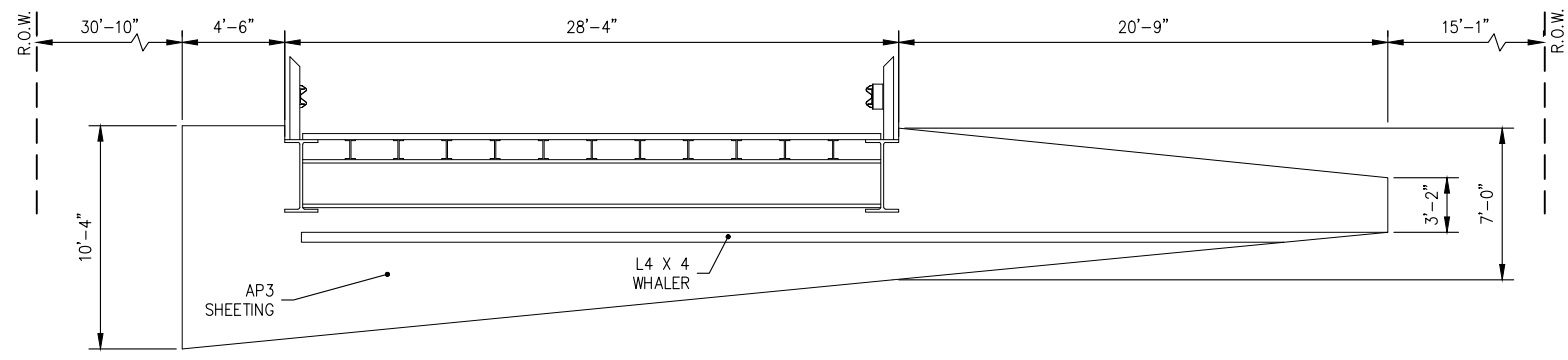
WEST TRANSVERSE ELEVATION NOT TO SCALE
