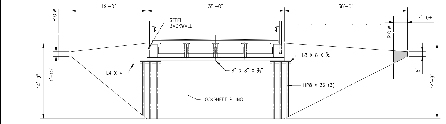
WEST TRANSVERSE ELEVATION
