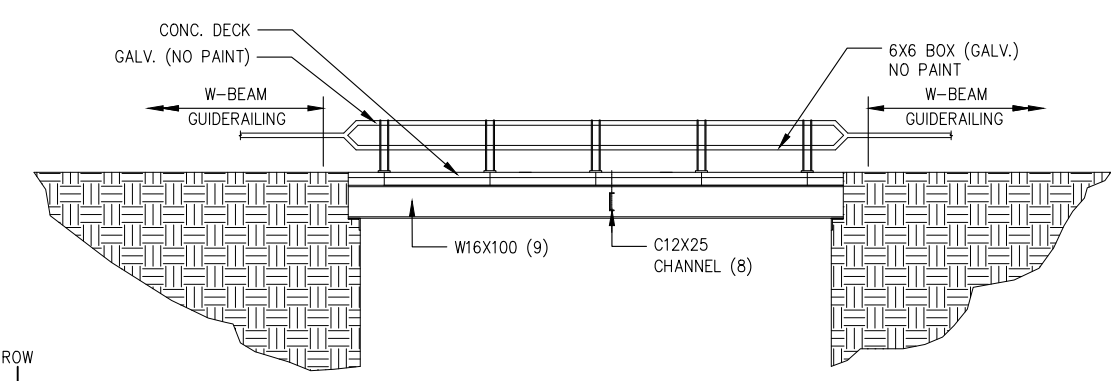
BRIDGE ELEVATION NOT TO SCALE
