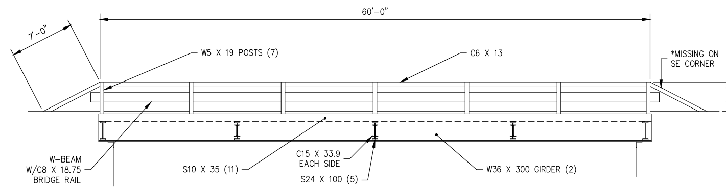
BRIDGE ELEVATION NOT TO SCALE
