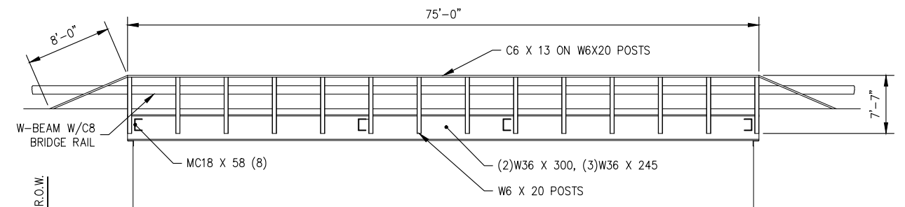
BRIDGE ELEVATION NOT TO SCALE
