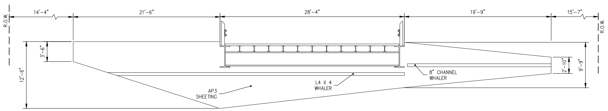
EAST TRANSVERSE ELEVATION NOT TO SCALE
