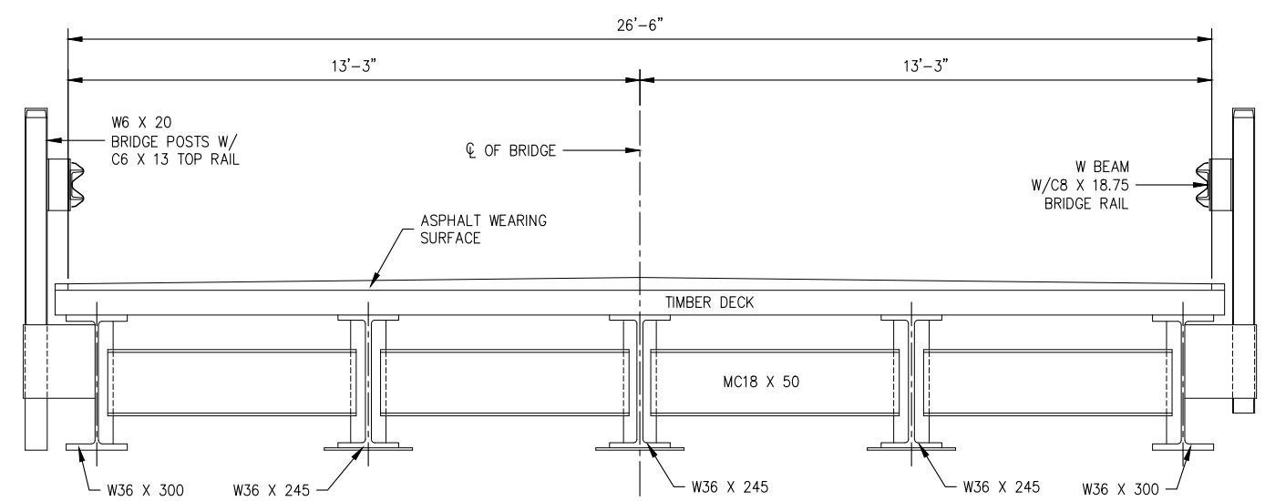
BRIDGE SECTION A-A NOT TO SCALE
