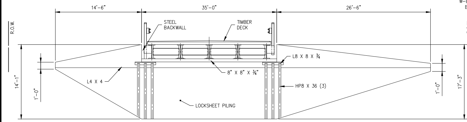
EAST TRANSVERSE ELEVATION NOT TO SCALE
