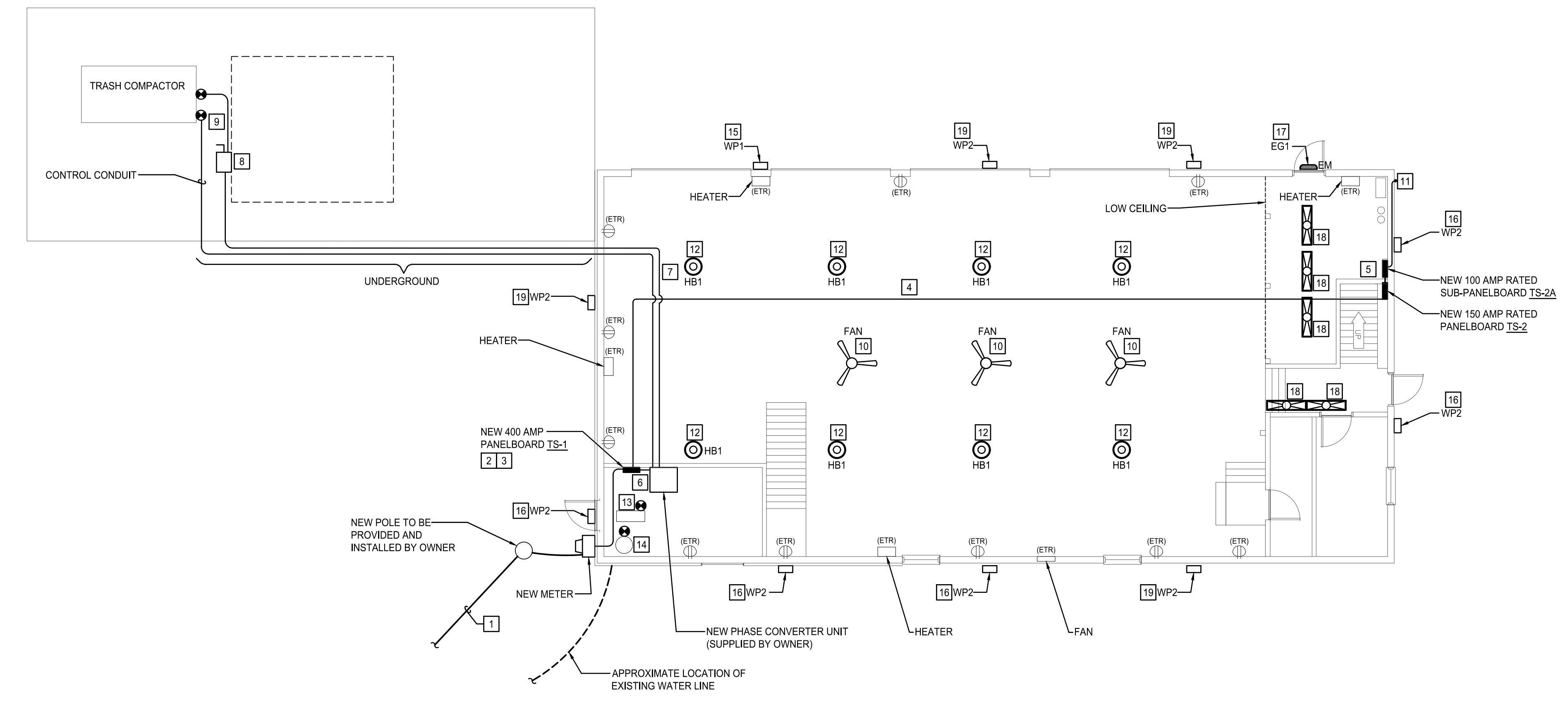
2 DPW BUILDING NEW WORK PLAN SCALE: 1/8" = 1' 0"
