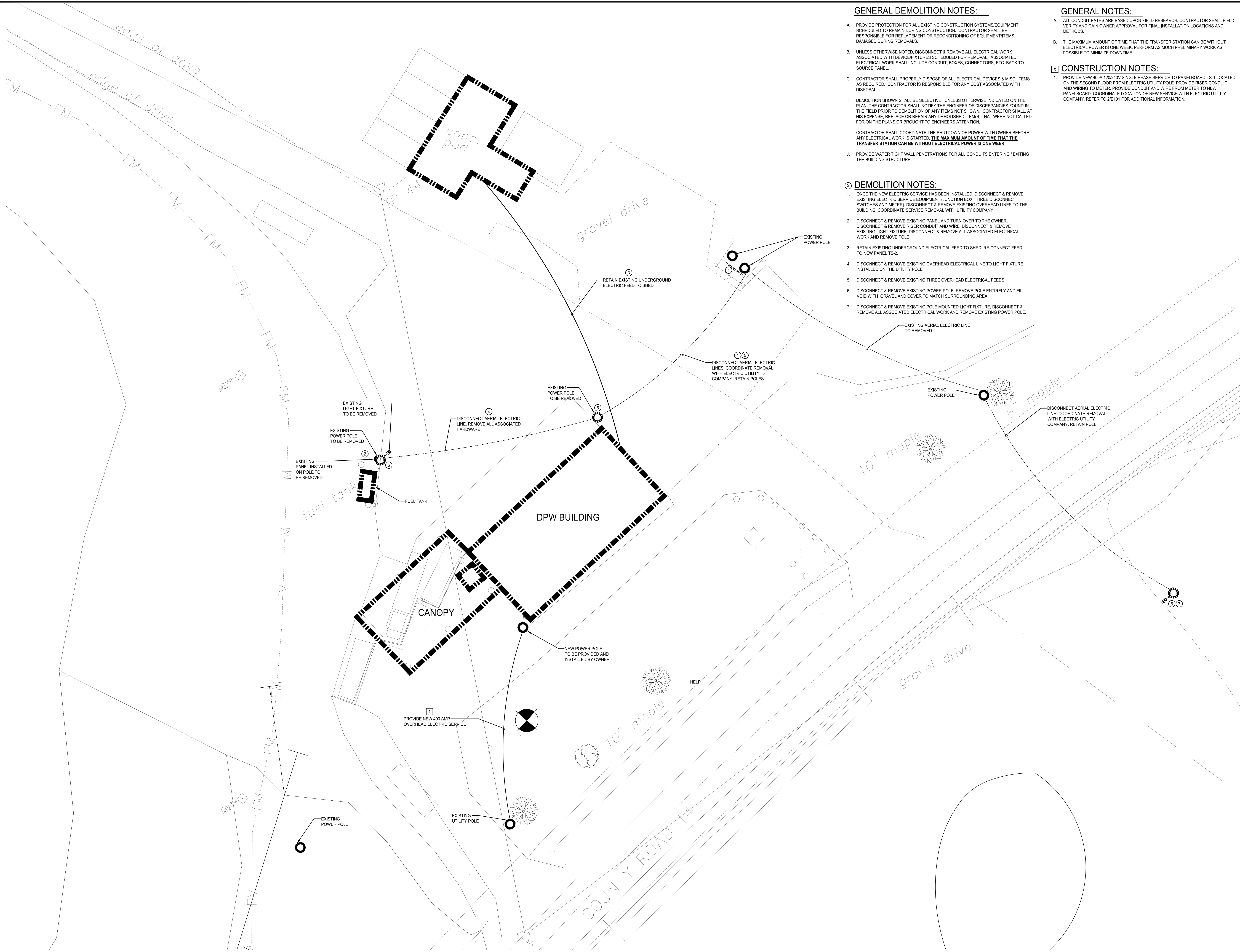
1 ELECTRICAL SITE PLAN SCALE: 1" = 15' 0"
