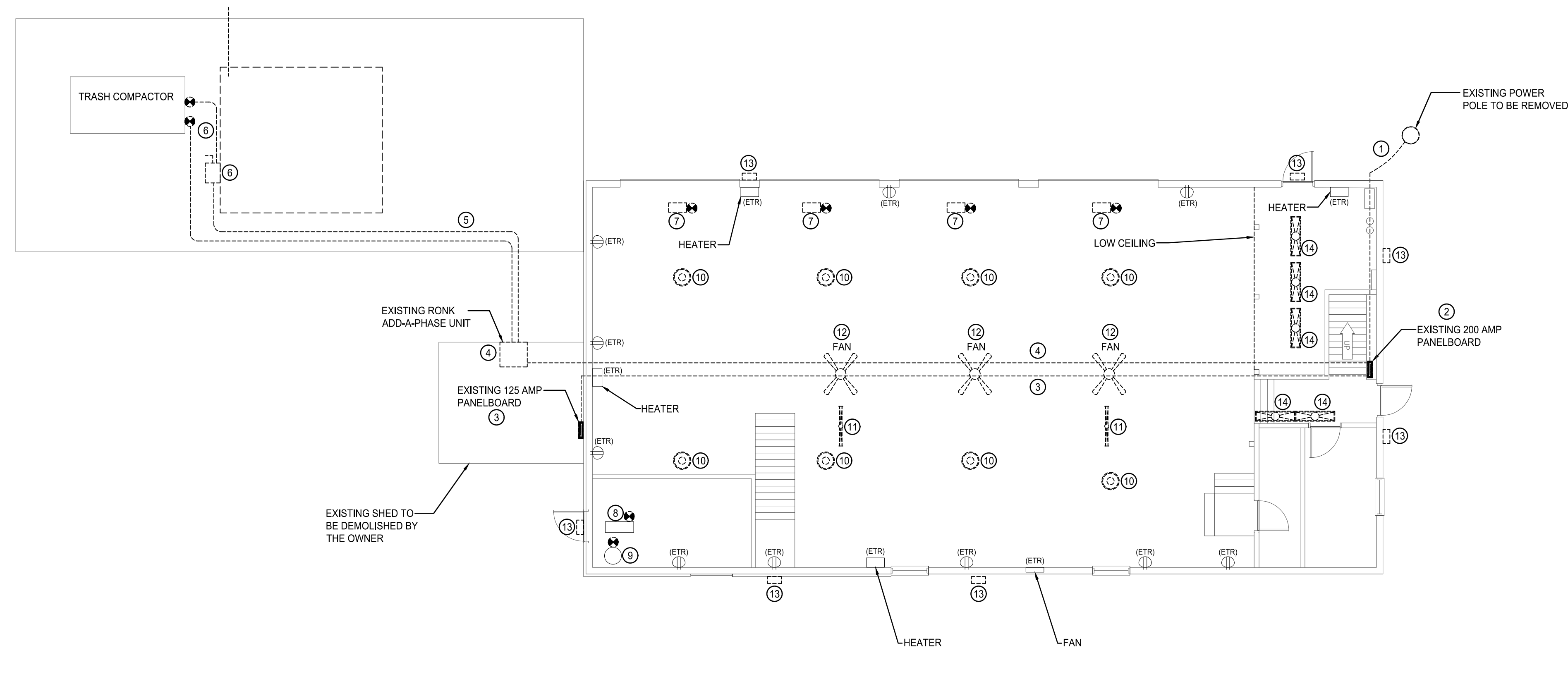
1 DPW BUILDING DEMOLITION PLAN SCALE: 1/8" = 1' 0"
