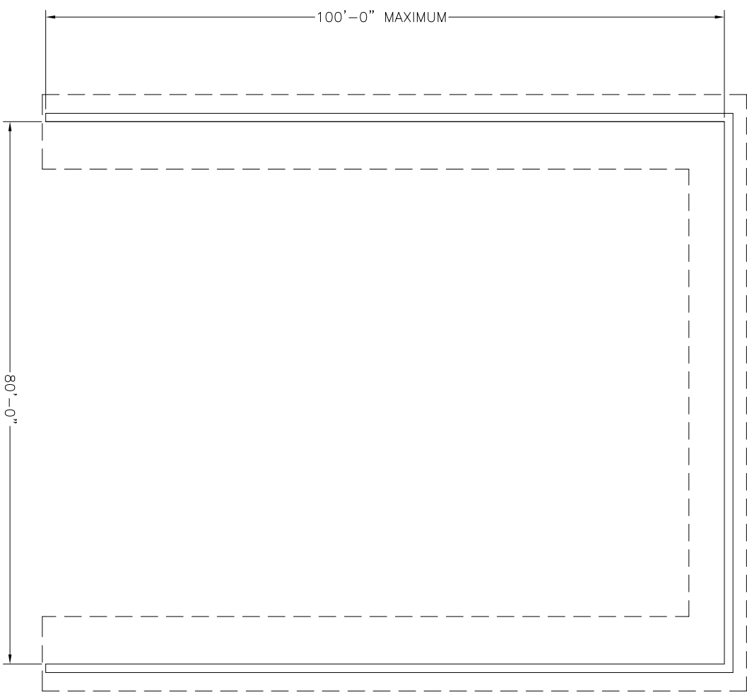
FOUNDATION PLAN SCALE: 1" = 10'-0"
