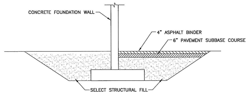
FOUNDATION BACKFILL SECTION
