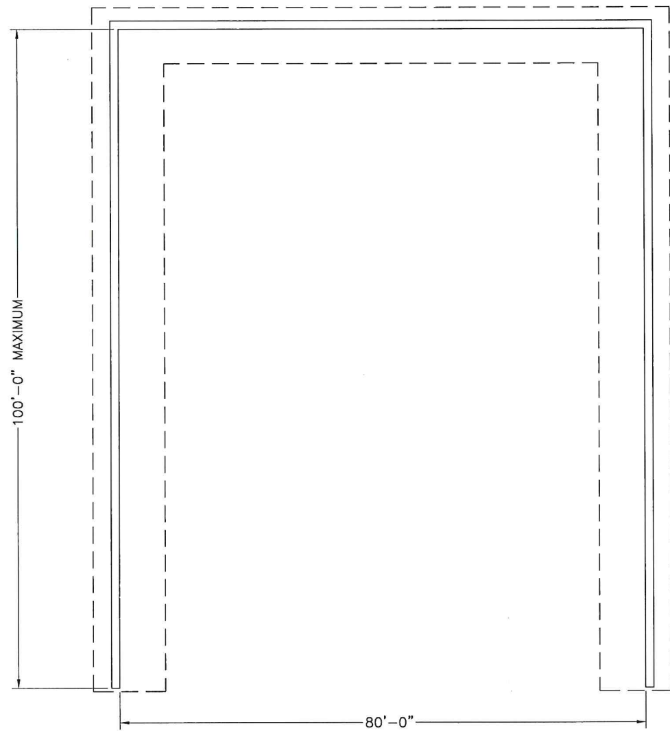
FOUNDATION PLAN
